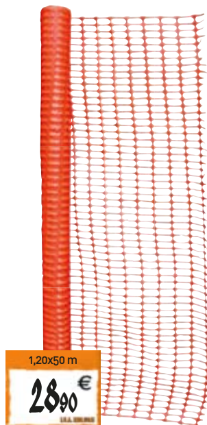
RETE ARANCIO DA CANTIERE 1,20x50 m, maglia 100x40 mm, 120 g 50132 € 28,90 1,80x50 m, maglia 100x26 mm, 140 g 50133 € 42,00
